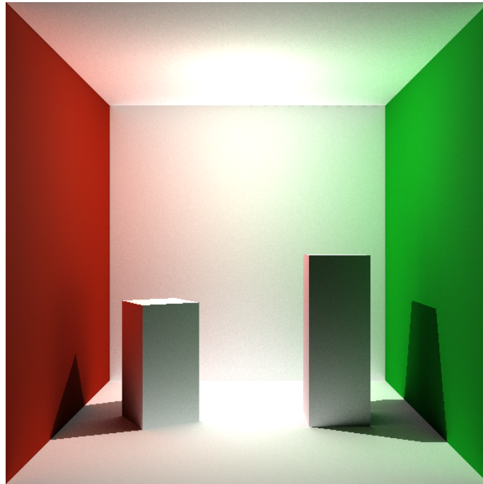
Figure 6.2: Example of point-based color bleeding without the volume extension algorithm.
