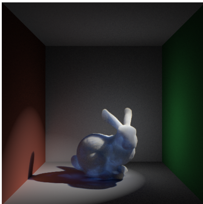
Figure 6.5: Image exemplifying clear color bleeding next to the red wall in the bunny's shadow and correct transmittance through the bunny's hollow form.
