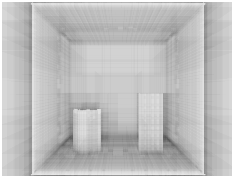
Figure 4.5: Illustrates the octree traversal algorithm testing efficiency. Lighter shades represent less tests, while darker shades represents the most. Closer objects evaluate faster, and all data in the point-cloud behind them are occluded.
