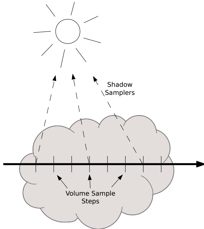
Figure 4.7: Stepping allows for estimation of the integral through the entire volume. Shadow rays are cast intermittently to estimate the direct lighting contribution.
