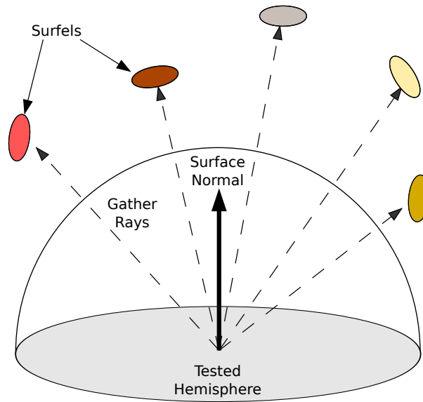
Figure 4.4: Gather rays are cast into the point-cloud, returning the estimated radiance coming from a given direction. The radiance is then scaled based on the solid angle of that sample cast (based on sample count.)
