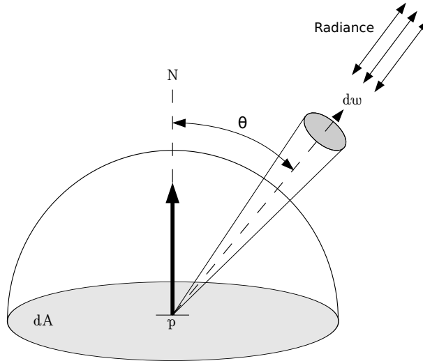
Figure 2.1: Evaluation of radiance at a point on an opaque surface. Only the hemisphere around the surface normal is considered. Incoming radiance is measured and scaled by its solid angle.
