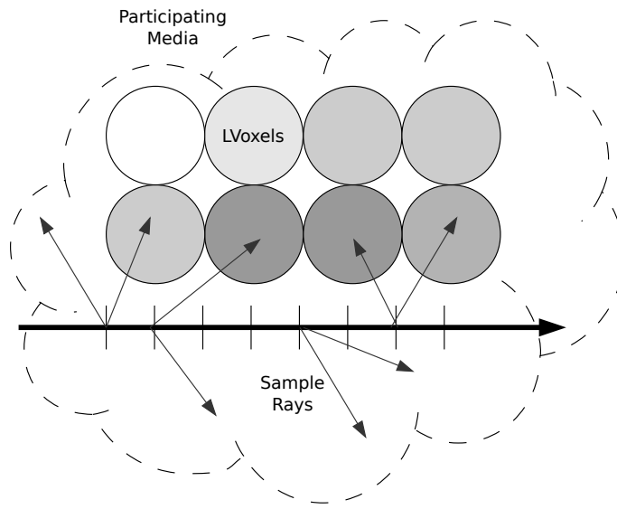
Figure 4.6: Sample rays are cast during volume traversal, allowing for decent estimates of lighting contribution at each point.
