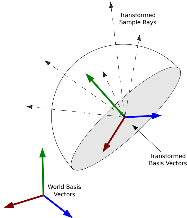
Figure 4.3: Basis vectors are generated based on the surface normal in order to transform samples on a hemisphere to test surrounding radiance.
