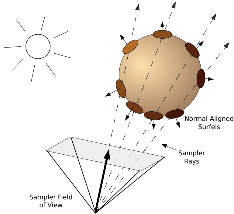
Figure 4.2: Rays are cast from a special camera during the surfel sample phase. Each time the ray intersects with geometry a surfel is created.
